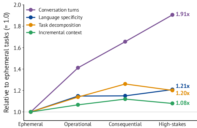
Figure 1: Critical work concentrates in advisory and professional domains, and task criticality shapes how people collaborate with AI. (a) Within-domain composition of task criticality for nine task domains, ranked by the Task Criticality Index (TCI; volume-weighted mean tier, 0–3). (b) Conversation turns, language specificity, task decomposition, and incremental context across the four criticality tiers, each shown relative to ephemeral tasks (=1.0). (c) Distribution of five engagement modes within each criticality tier, as a share of conversations in that tier.
