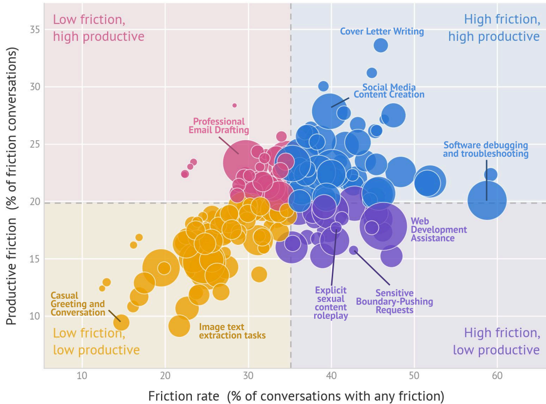
Figure 5: The relationship between friction prevalence and friction productivity varies across task types. Each point represents a cluster, plotted by the rate at which friction occurs (x-axis) and the proportion of friction conversations that are productive (y-axis). The bubble size reflects the number of conversations within each cluster. It is worth noticing that although consequential tasks and high-stakes tasks are likely to have higher prevalence of friction, this friction also yields productive outcomes as 40.8% of these tasks fall in the top-right quadrant.
