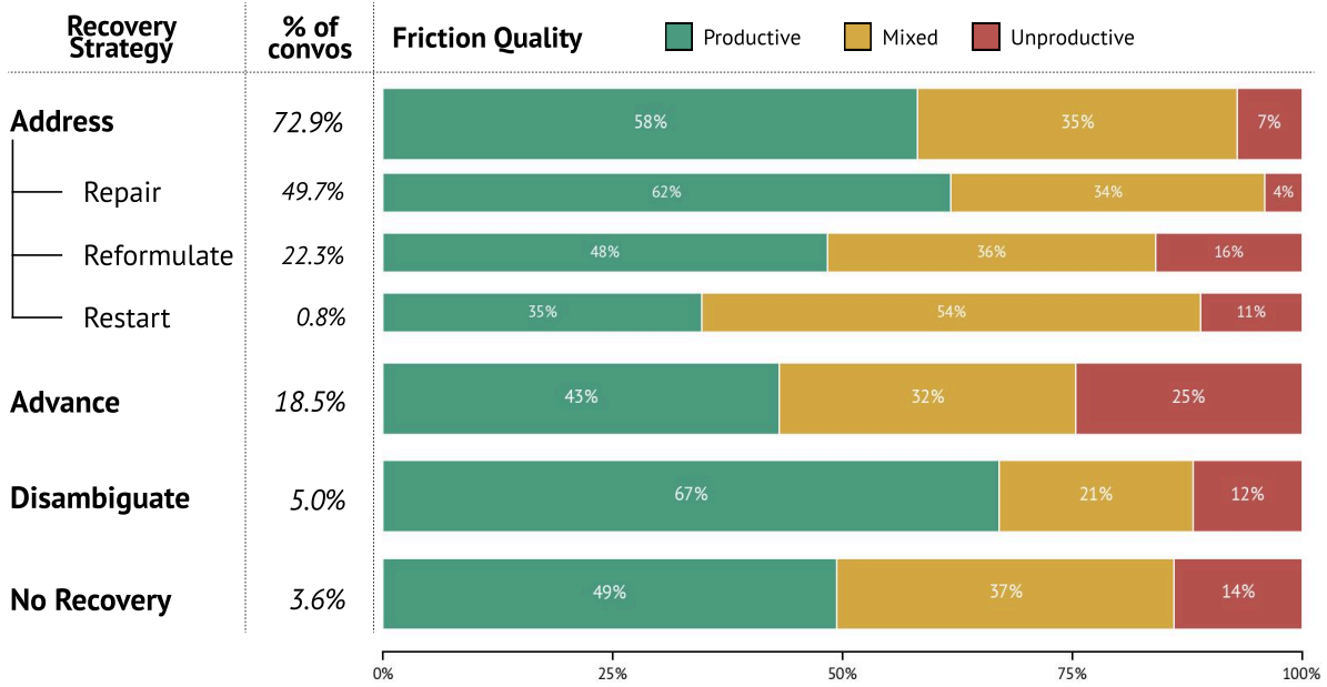
Figure 6: Users employ active strategies to address friction in interaction. We show the frequency that each recovery strategy was employed as a percentage out of conversations that contain friction. For each category, we plot the distribution of conversations that ended productively, unproductively, and mixed. Addressing acts are the most commonly employed recovery strategy, covering 72.9% of conversations. Within this category, users are more likely to attempt to directly repair misalignments (49.7%) compared to trying reformulations of their initial prompt (22.3%).
